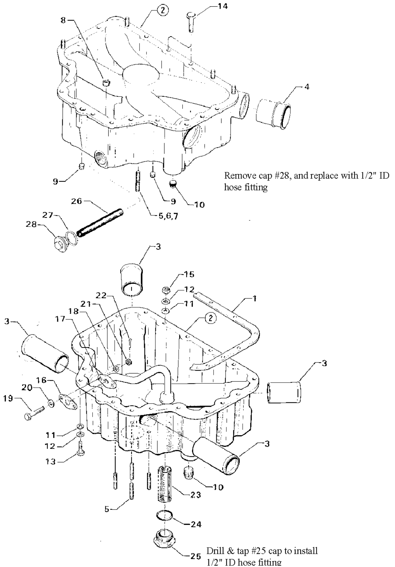
Figure 28. OIL SUMP ASSEMBLY AND OIL SUCTION SCREEN
